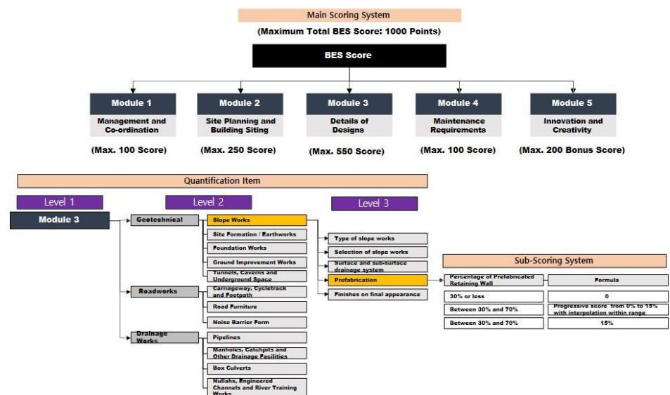
Figure 5. A schematic diagram of the quantification item and method for BES.
